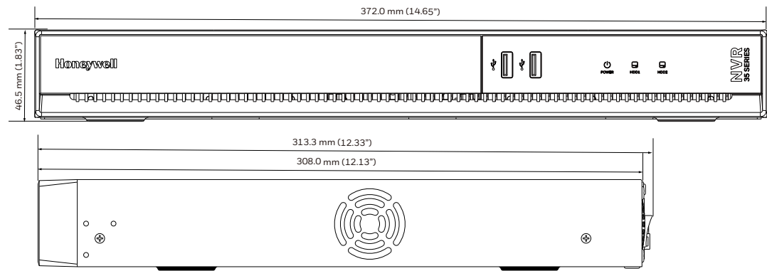
HN350802xxC/HN351602xxC
