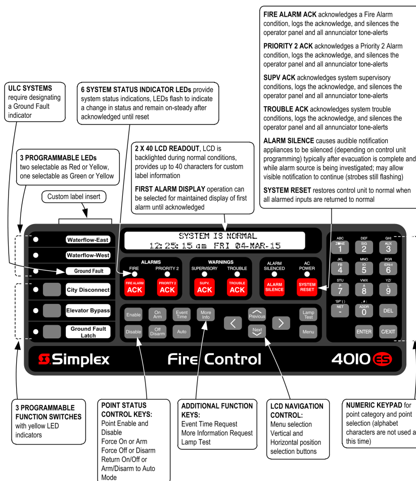
Figure 11: Operator interface
