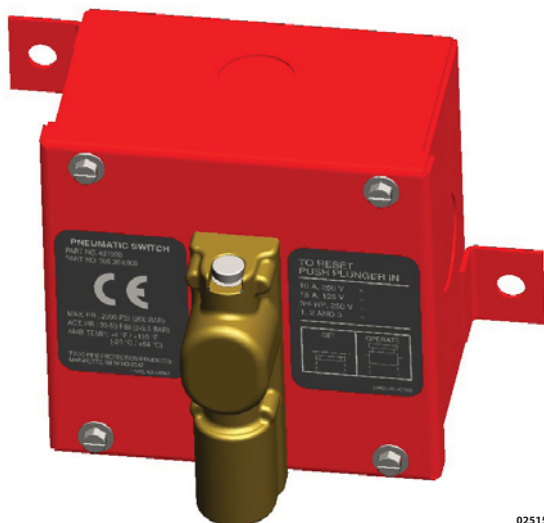
Figure 36 - Discharge Pressure Switch (Part No. 437900)
